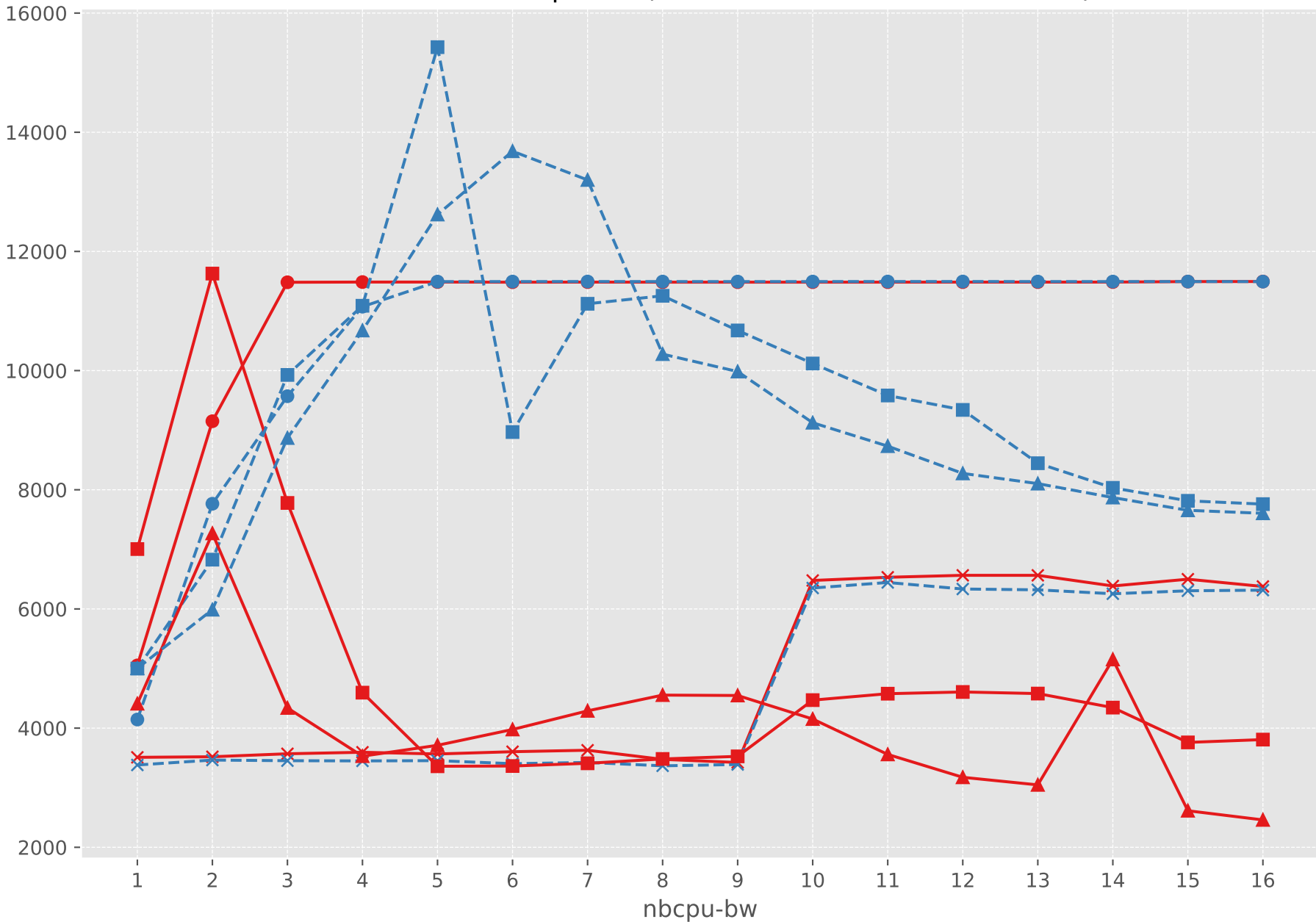
Bandwidth vs nbcpu-bw (CPU vs DPU, Direct vs Buffered)
